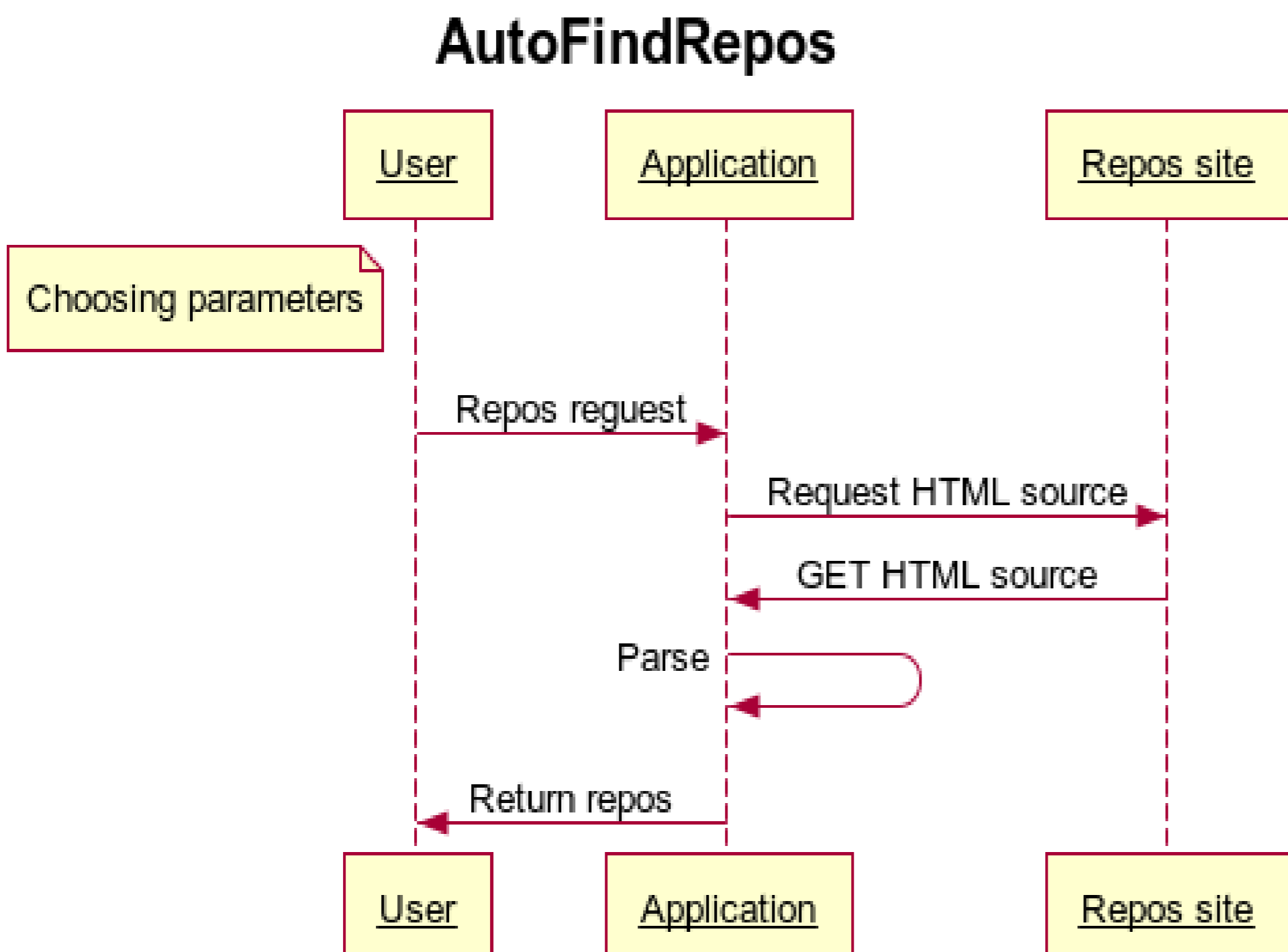
Sequence diagram
